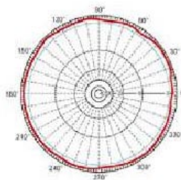
H-Plane Co-polarization 3-dB Beam width = 360°
